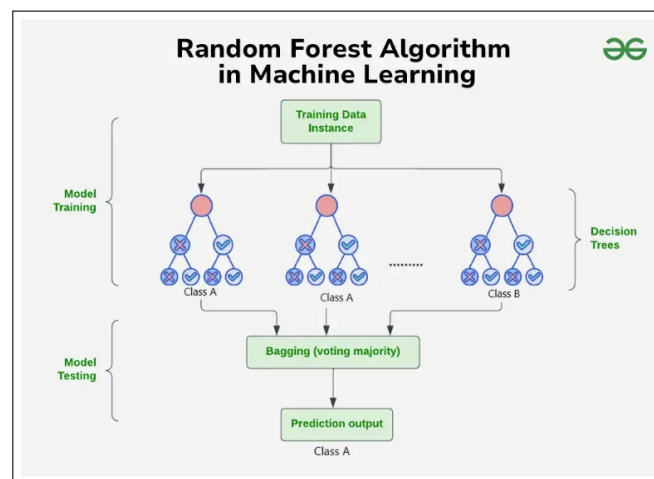
Figure 1: Random Forest Algorithm.
