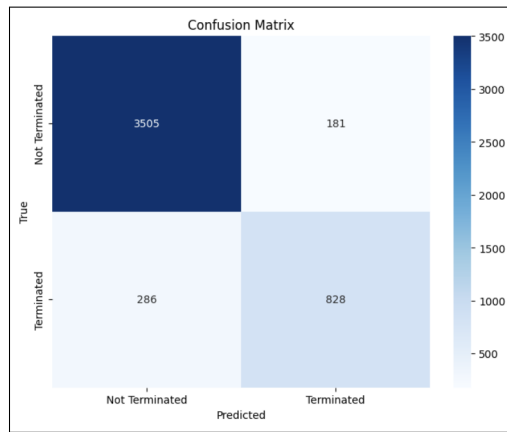
Figure 3: Confusion matrix.
